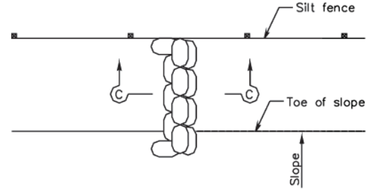
CROSS BARRIER DETAIL
